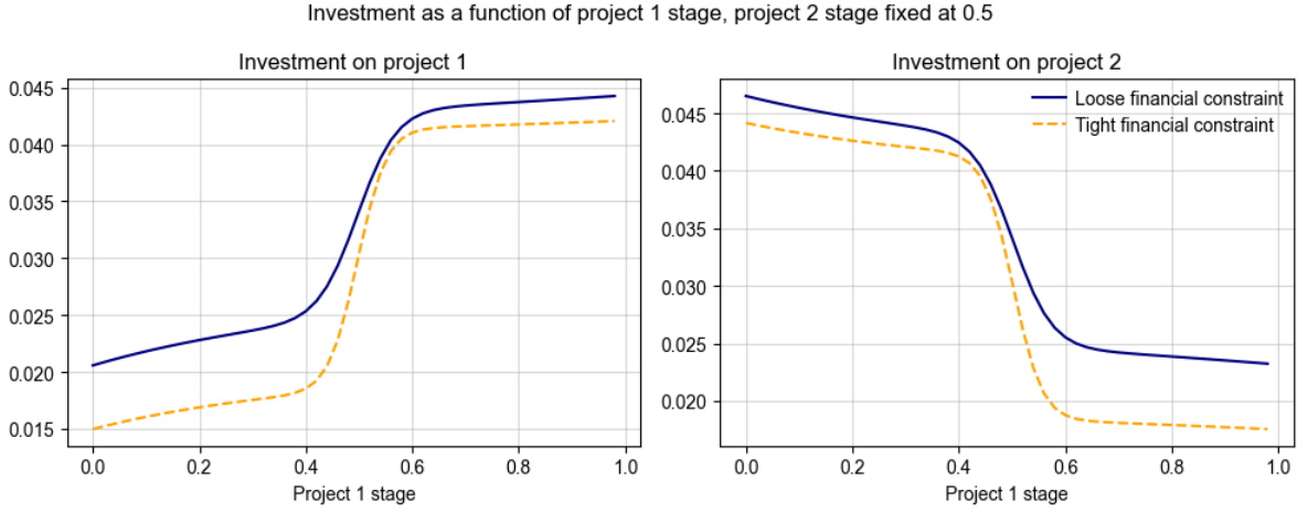
Figure A20: Optimal Investment with Spending Constraints
